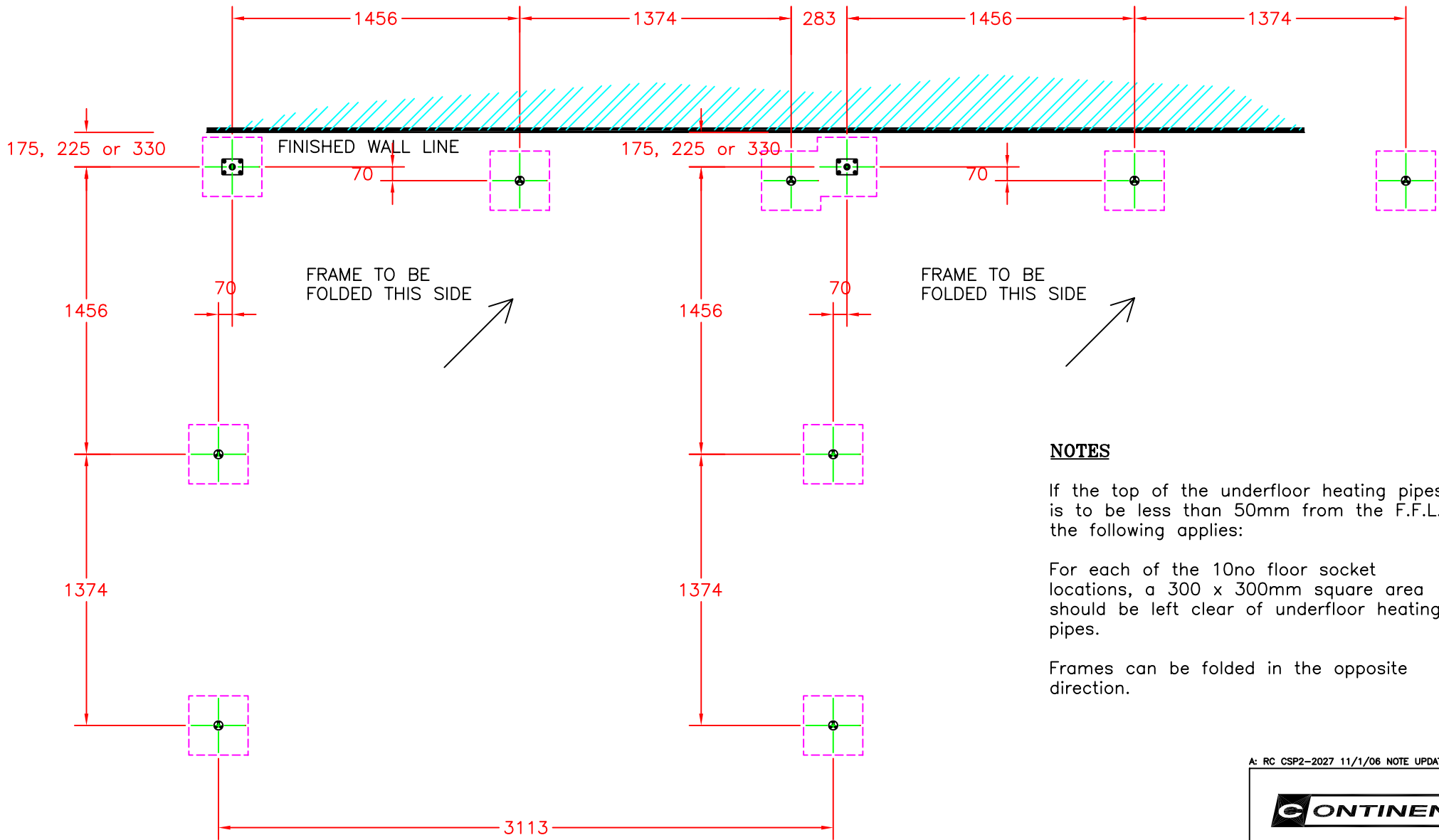
LOCATION PLAN
