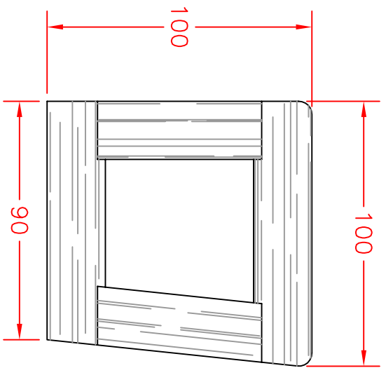
SIDE BOARD CROSS SECTION (Scale 1:2)
