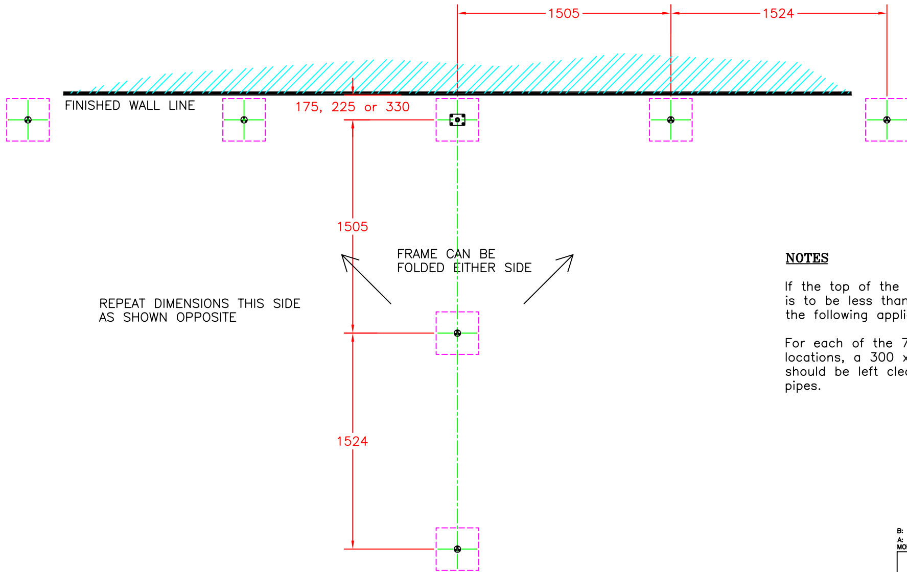
LOCATION PLAN
