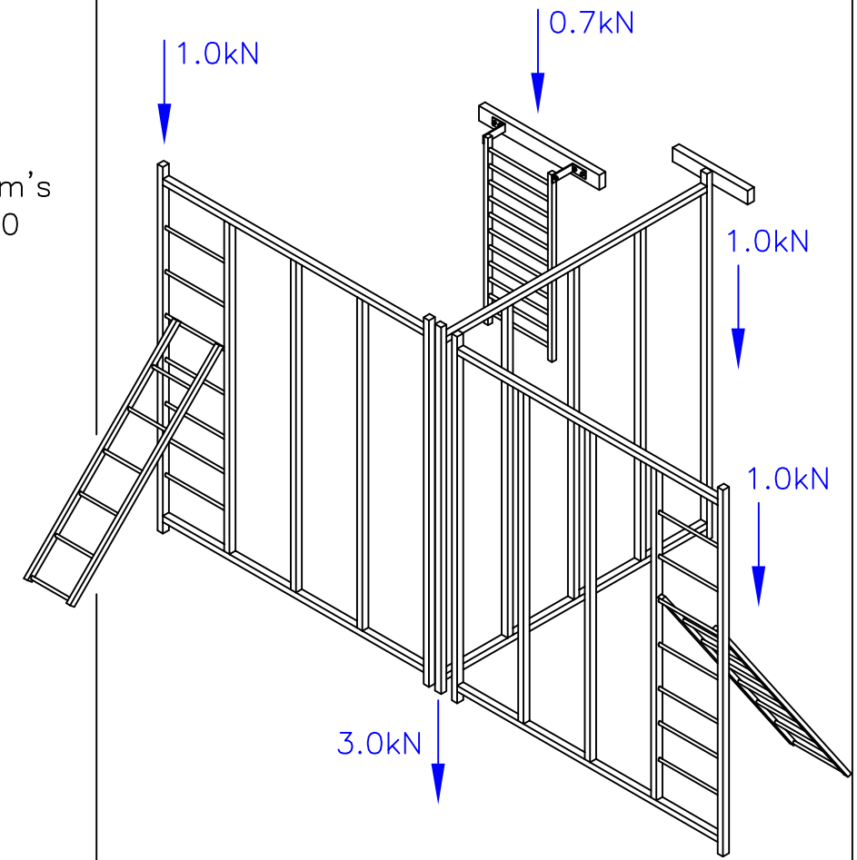
3D VIEW OF THE CLIMBING FRAME
