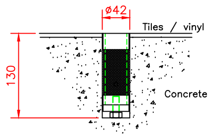
Solid Floor Socket Details
